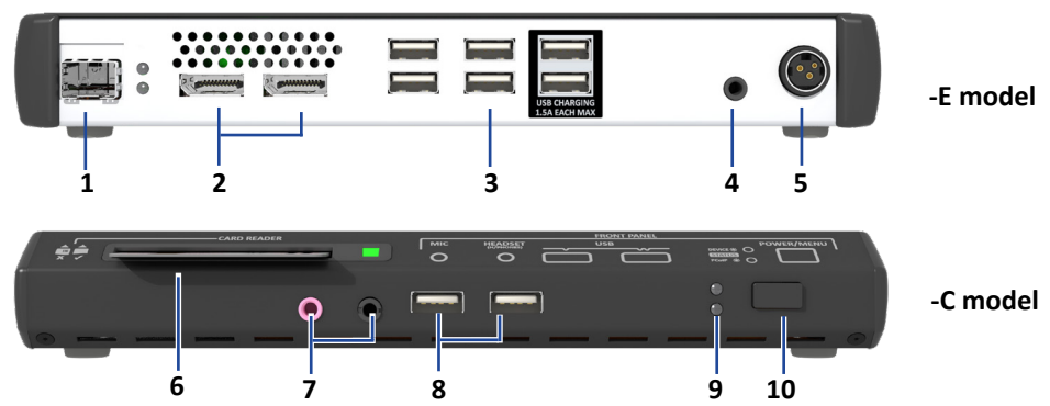
1 Network port. 2 DisplayPort connectors. 3 USB ports (two for high charge-current devices). 4 Line-level audio output. 5 DC power inlet. 6 Card reader. 7 Mic and headset sockets. 8 Easy access USB. 9 LED indicators. 10 Power/Menu switch.
