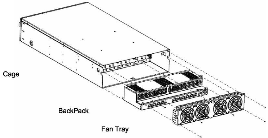
Cage/BackPack/Fan Tray Assembly Diagram
